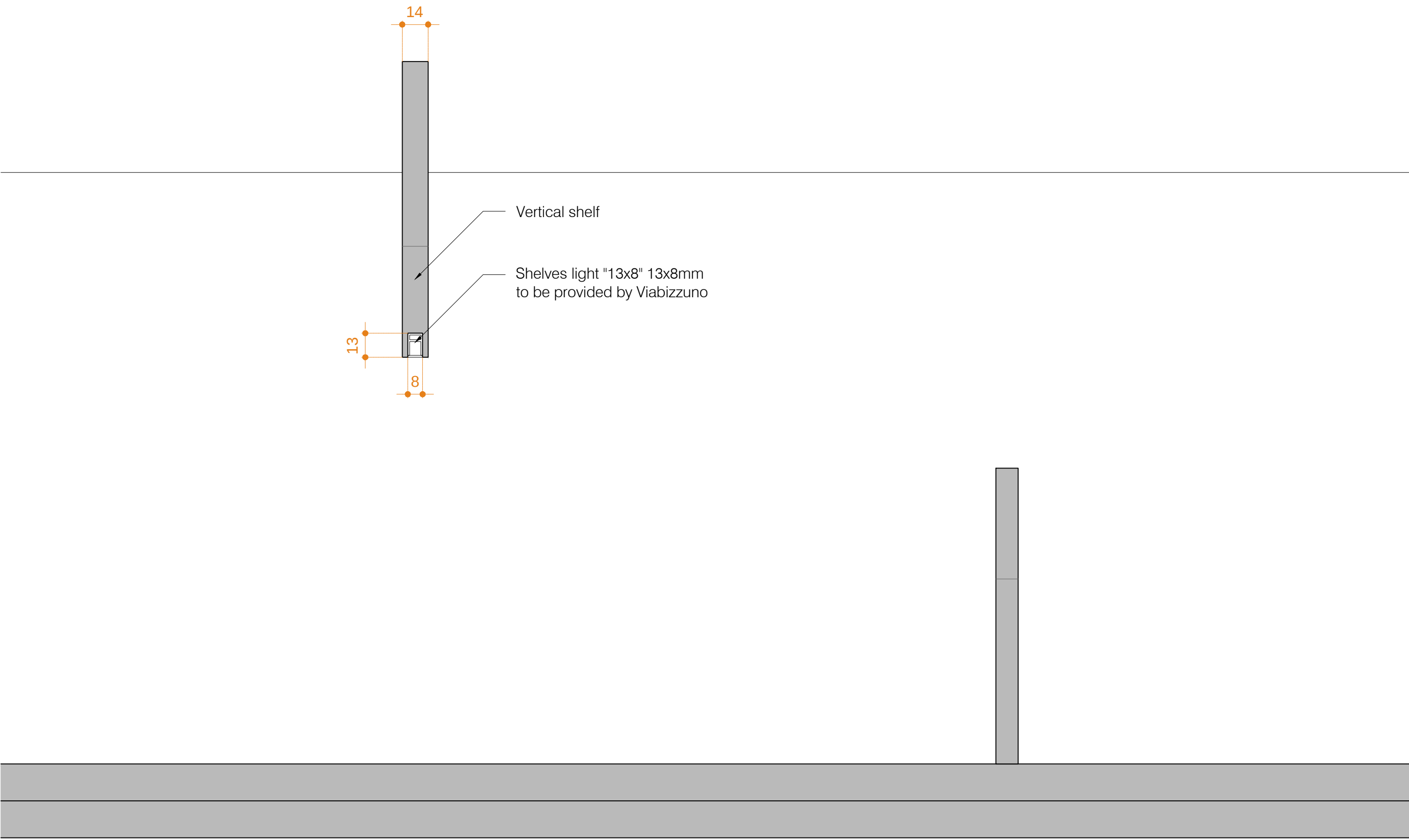
Shelves light - detail section ::: e 1/2
