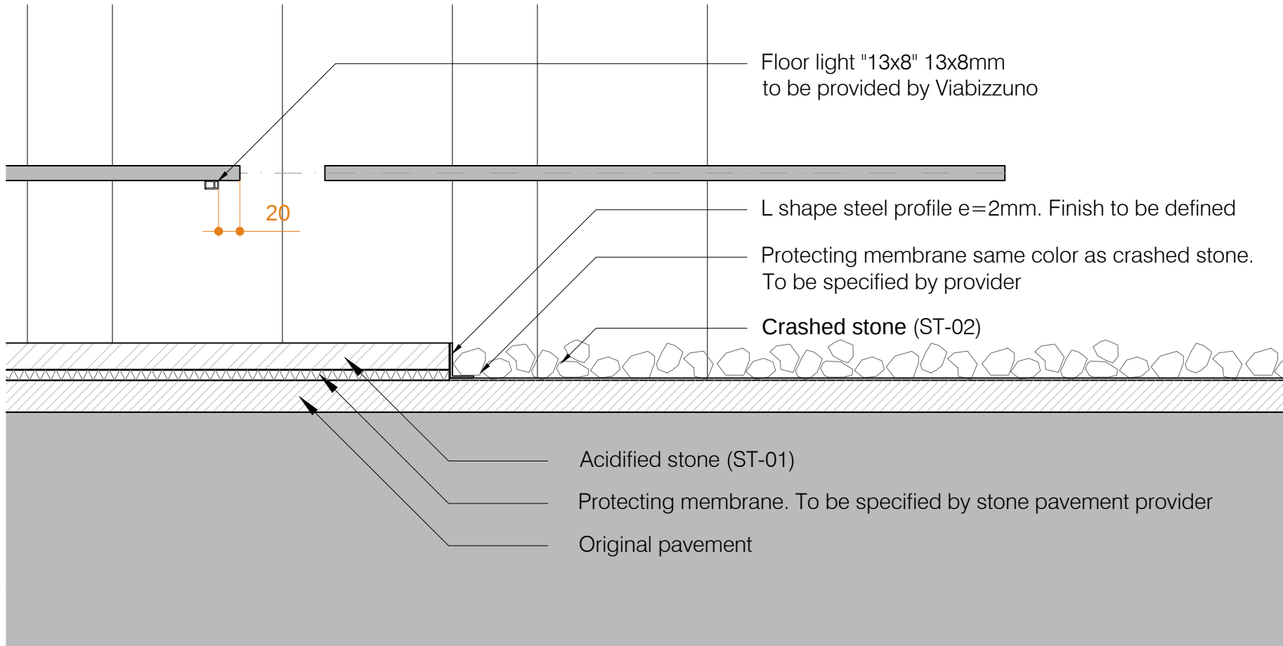
Section 3 ::: e 1/5
