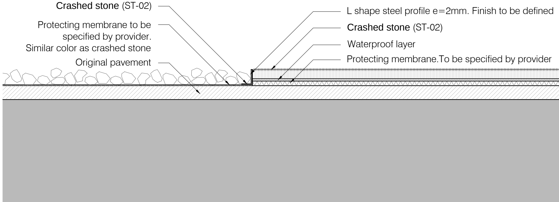
Section 4 ::: e 1/5
