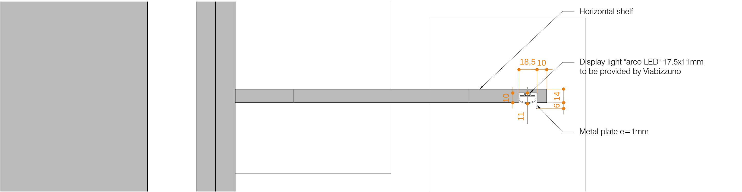
Display light - detail section ::: e 1/2
