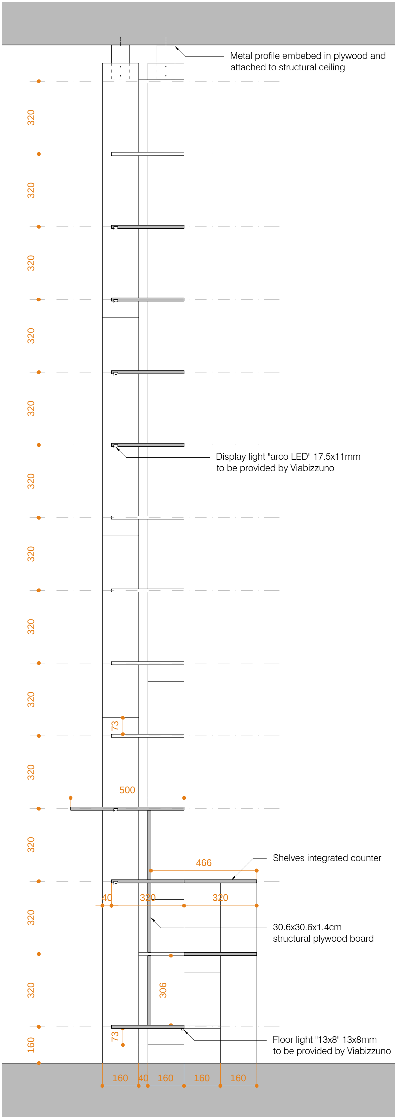
Section 2 ::: e 1/10
