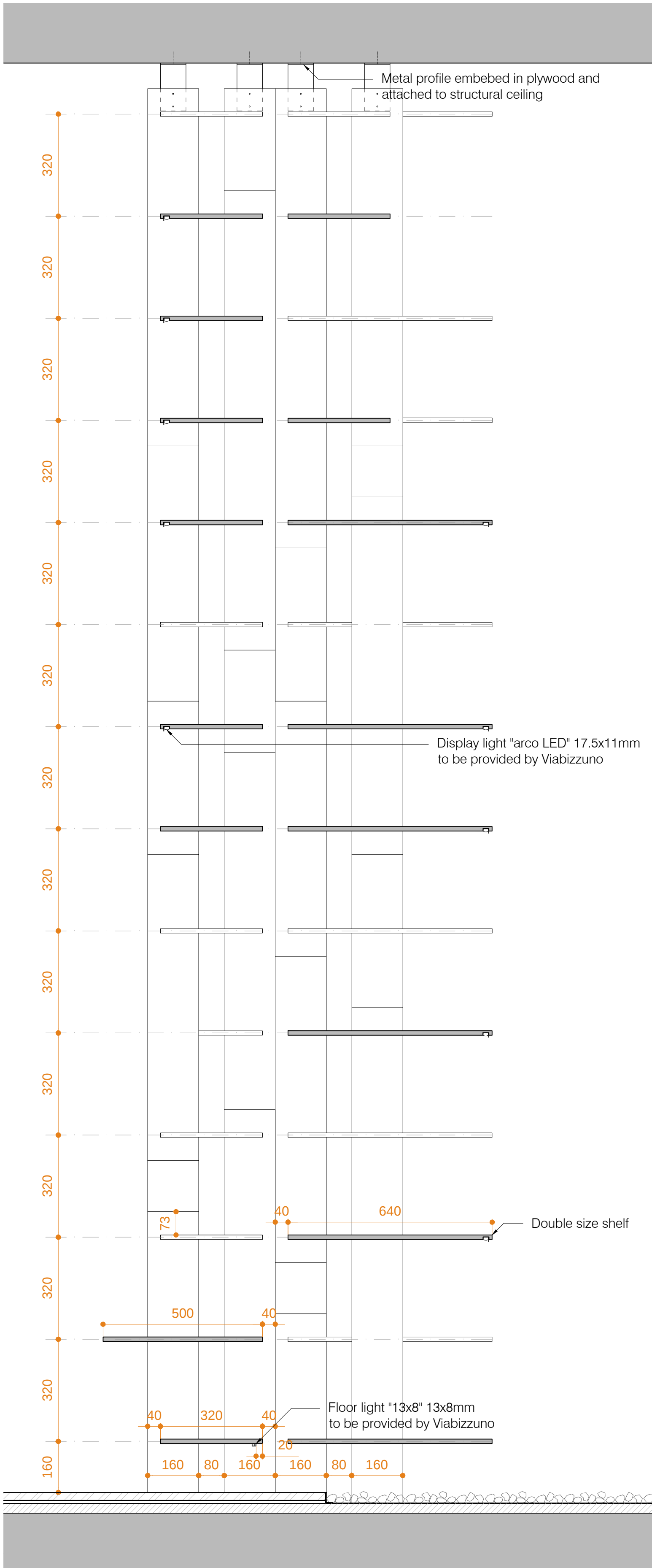
Section 3 ::: e 1/10
